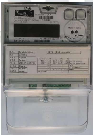
Figure 2.1 E11x meter – front view
