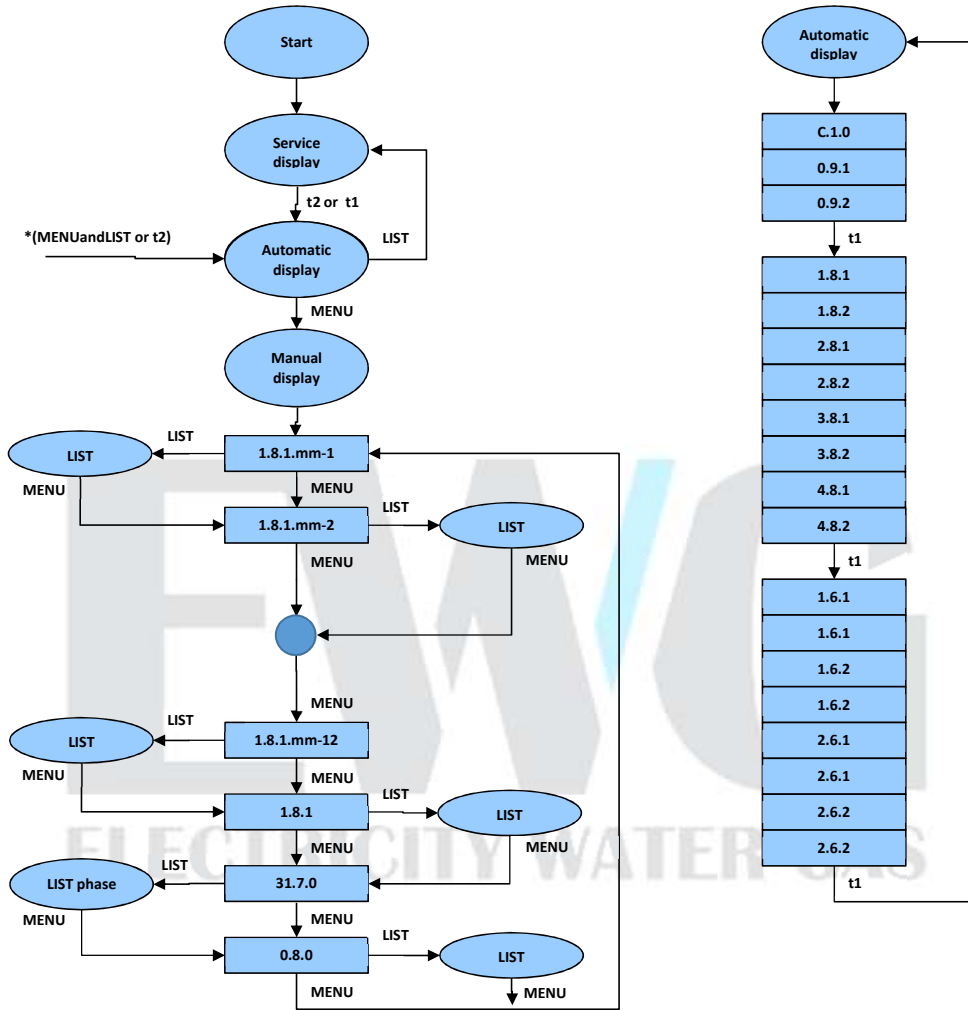
Figure 4.2 Display navigation diagram
