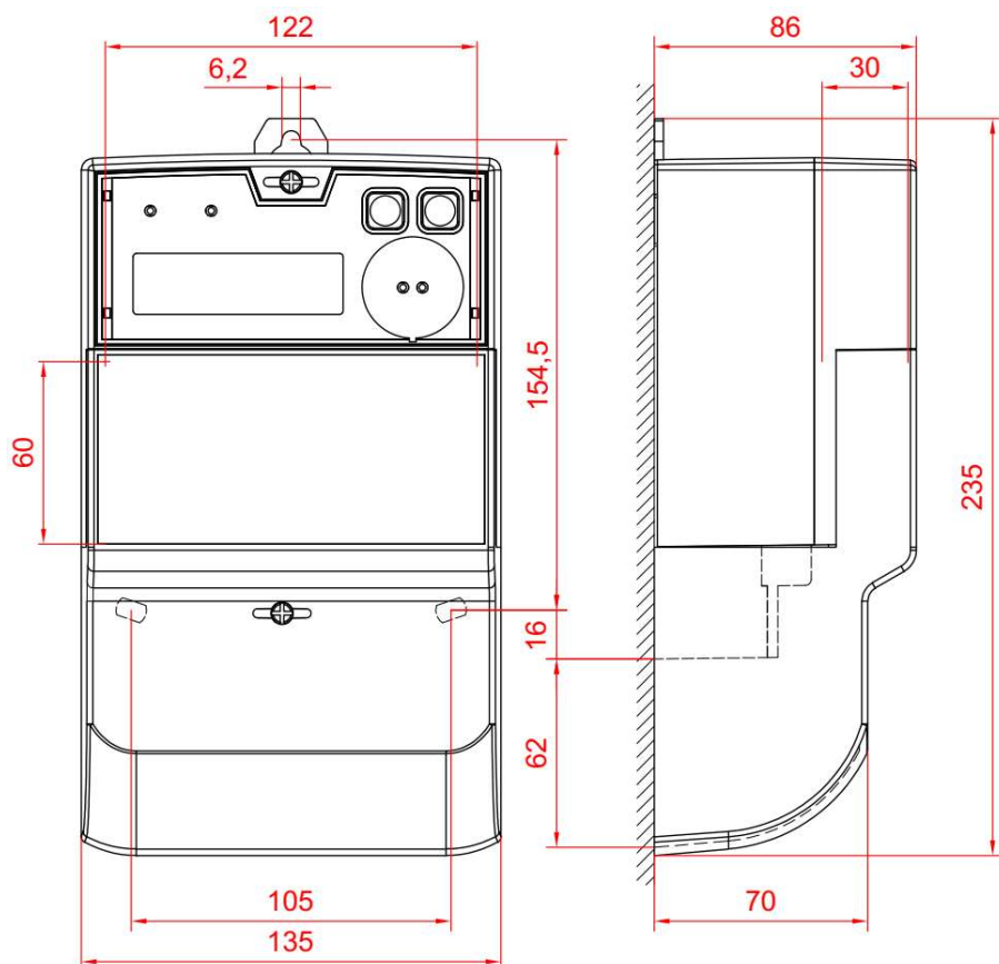
Figure 2.2. Dimensions of the meter
