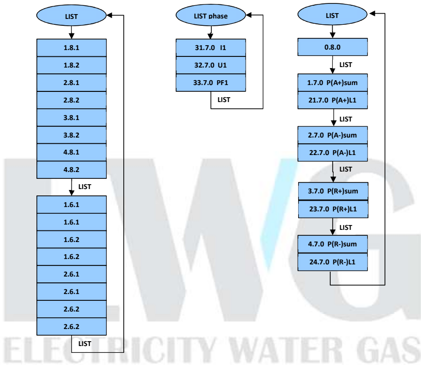
Figure 4.3 Display navigation diagram – manual mode
