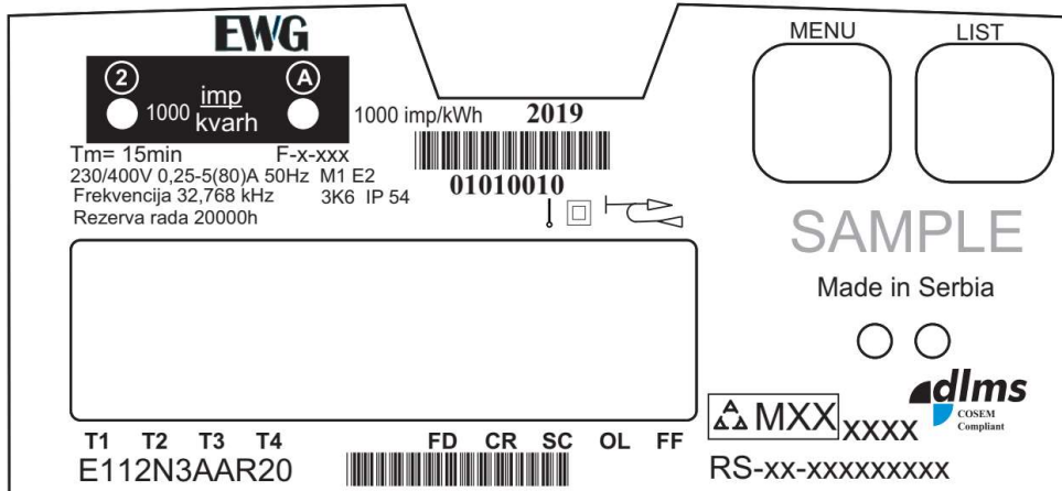
Figure 2.5 Name plate E11xxx
