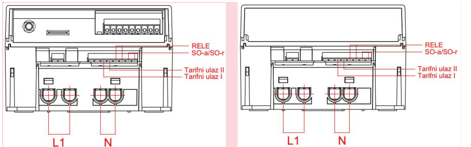
Figure 2.4. Meter terminal connector's labels (with GPRS module left, without module right)
