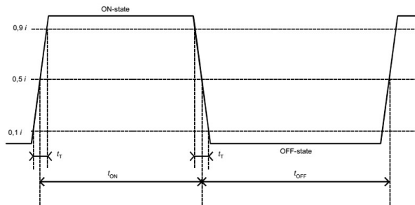
Picture 3.2 Waveform of the optical test output
