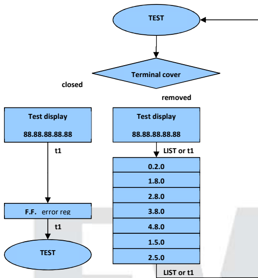
Figure 4.4 Display navigation diagram – test mode
