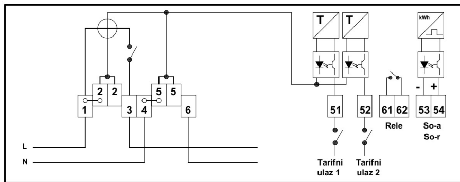
Figure 2.7 Single-phase direct connected meter scheme
