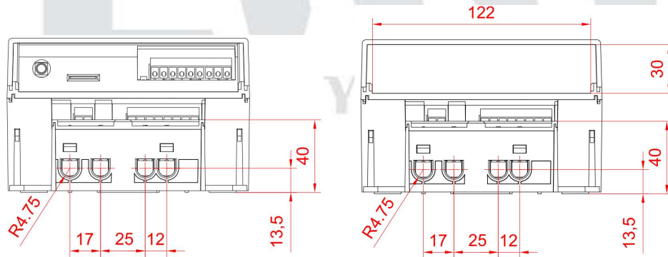
Figure 2.3 Meter terminal dimensions (with GPRS module left, without module right)
